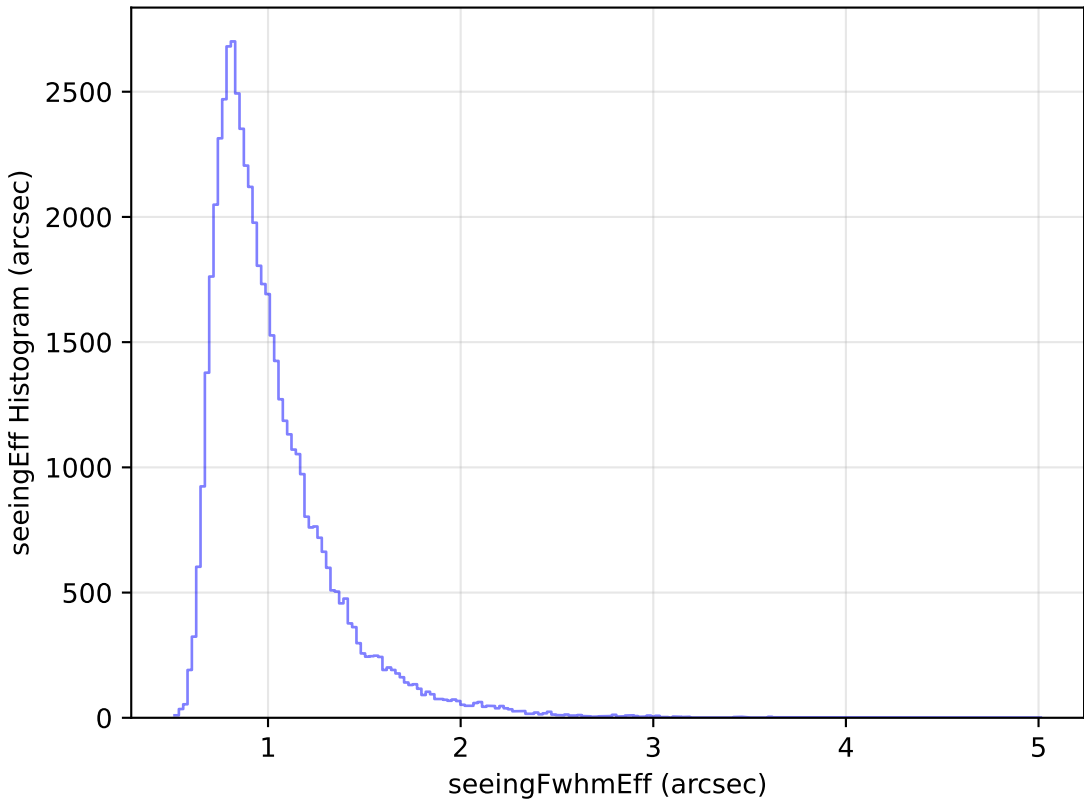
too_elab_heavy_r64_d3_gz_v3.4_10yrs Yr 1 i band: seeingEff Histogram
