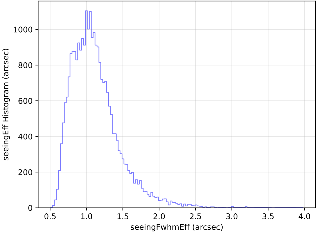
too_elab_heavy_r64_d3_gz_v3.4_10yrs Yr 1 g band: seeingEff Histogram
