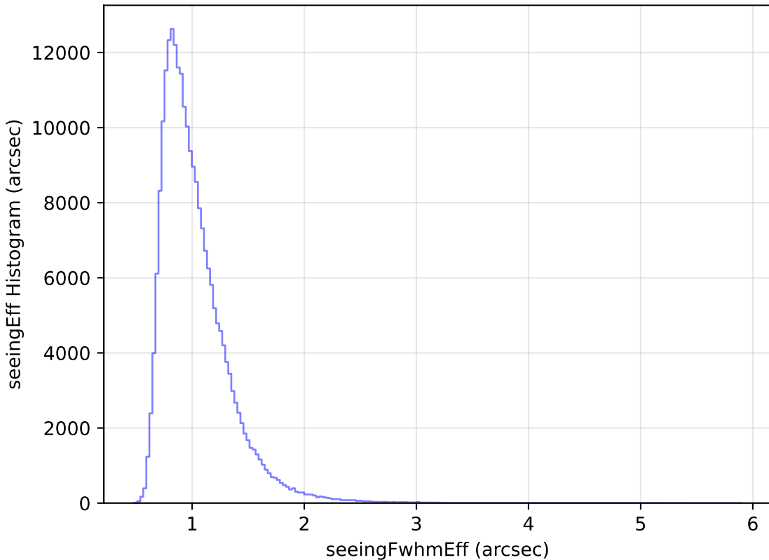
too_elab_heavy_r64_d3_gz_v3.4_10yrs Yr 1 all bands: seeingEff Histogram
