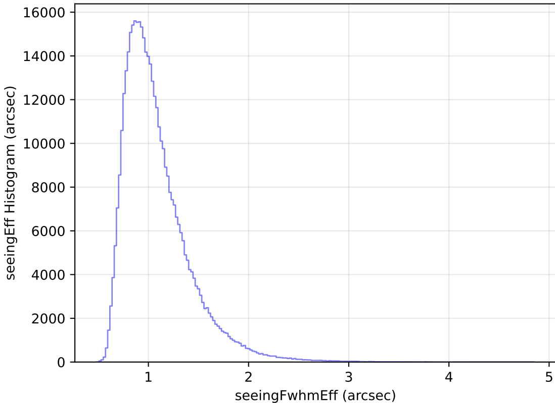
too_elab_heavy_r64_d3_gz_v3.4_10yrs WFD z band: seeingEff Histogram
