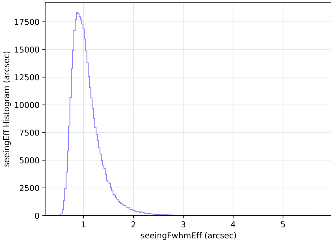
too_elab_heavy_r64_d3_gz_v3.4_10yrs WFD y band: seeingEff Histogram
