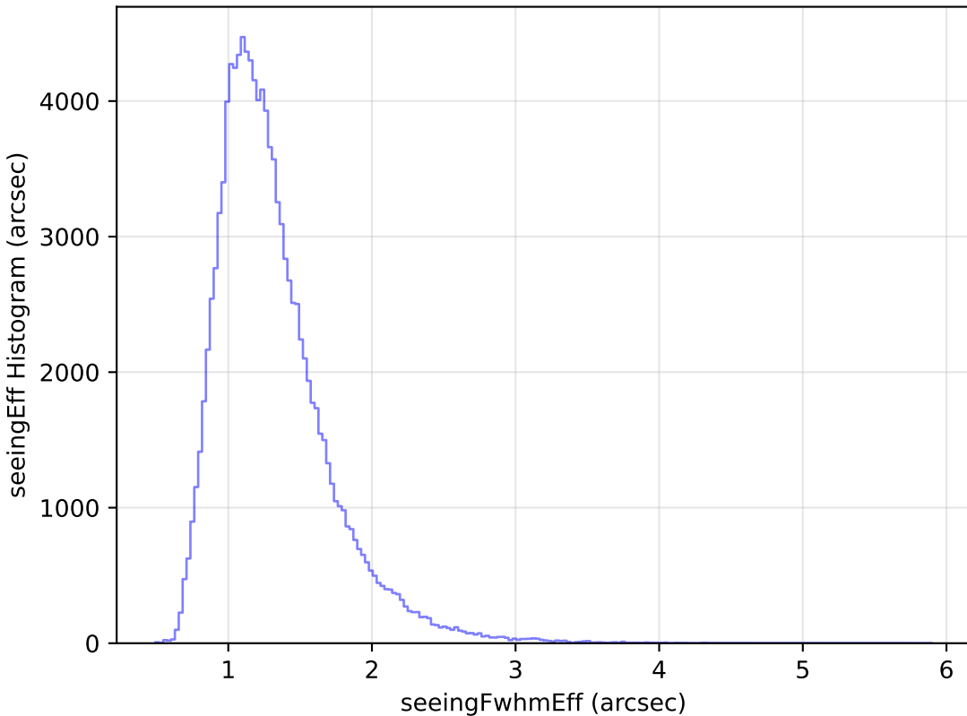
too_elab_heavy_r64_d3_gz_v3.4_10yrs WFD u band: seeingEff Histogram
