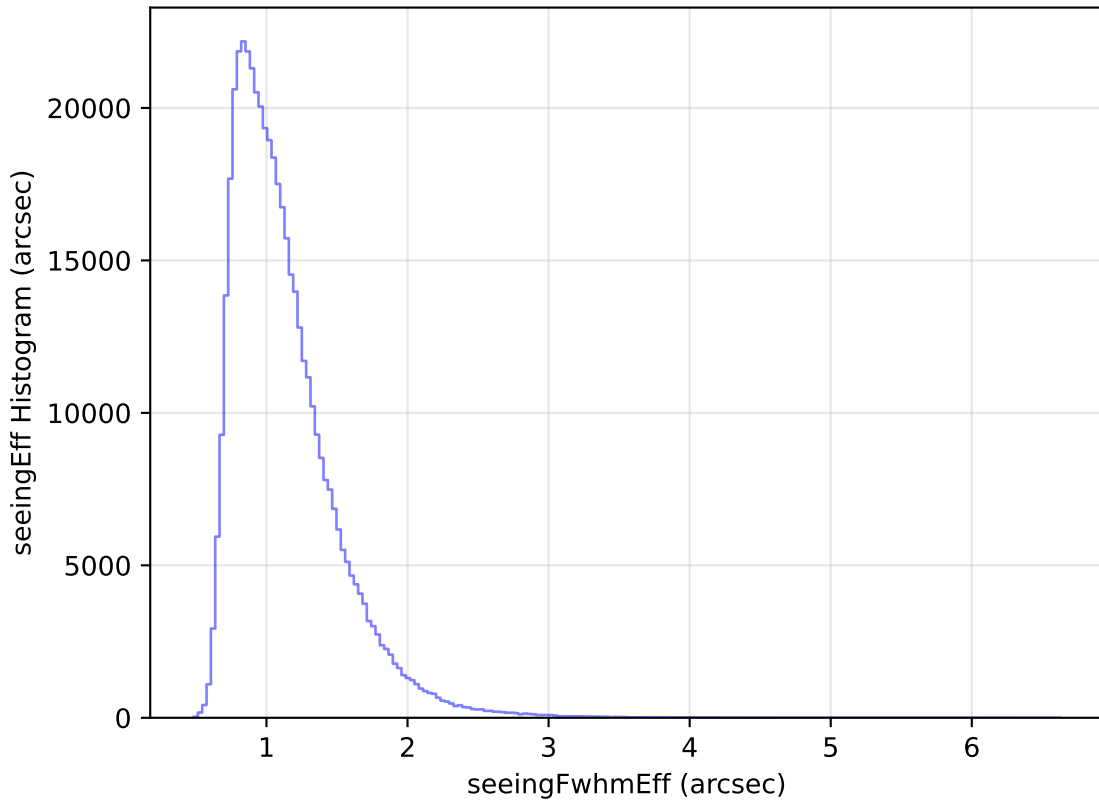
too_elab_heavy_r64_d3_gz_v3.4_10yrs WFD r band: seeingEff Histogram
