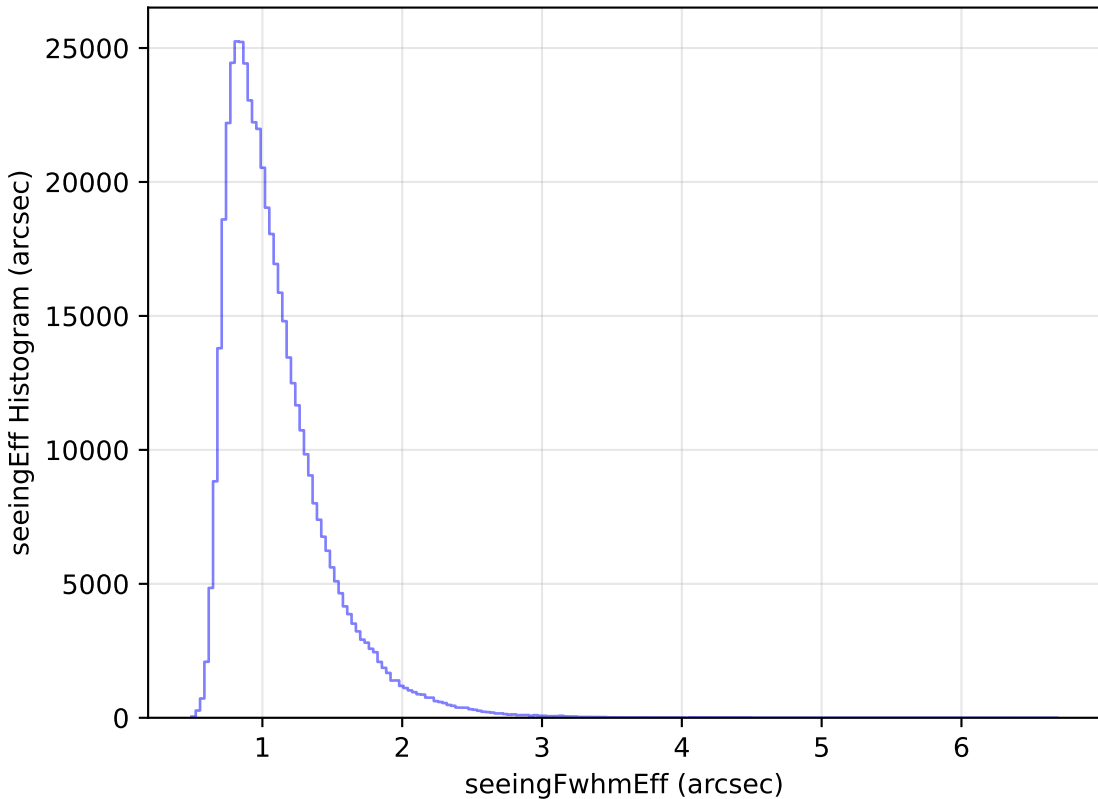
too_elab_heavy_r64_d3_gz_v3.4_10yrs WFD i band: seeingEff Histogram
