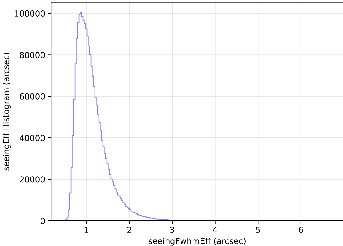
too_elab_heavy_r64_d3_gz_v3.4_10yrs WFD all bands: seeingEff Histogram
