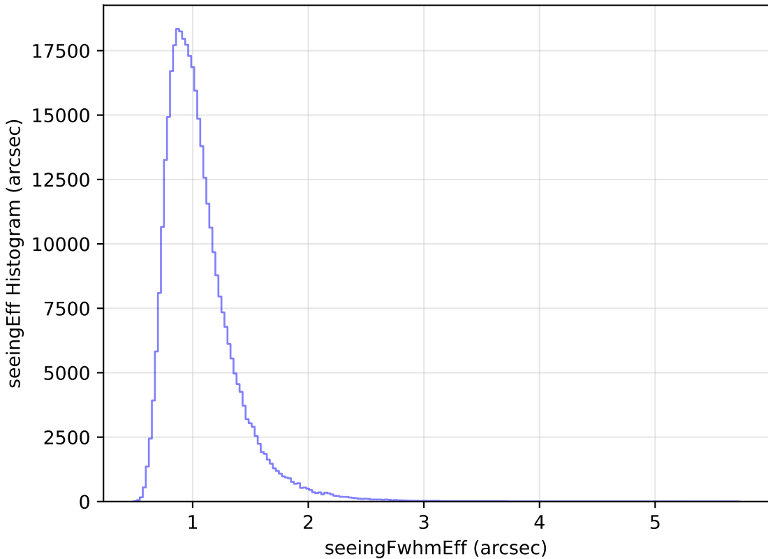
too_elab_heavy_r64_d3_gz_v3.4_10yrs All sky y band: seeingEff Histogram
