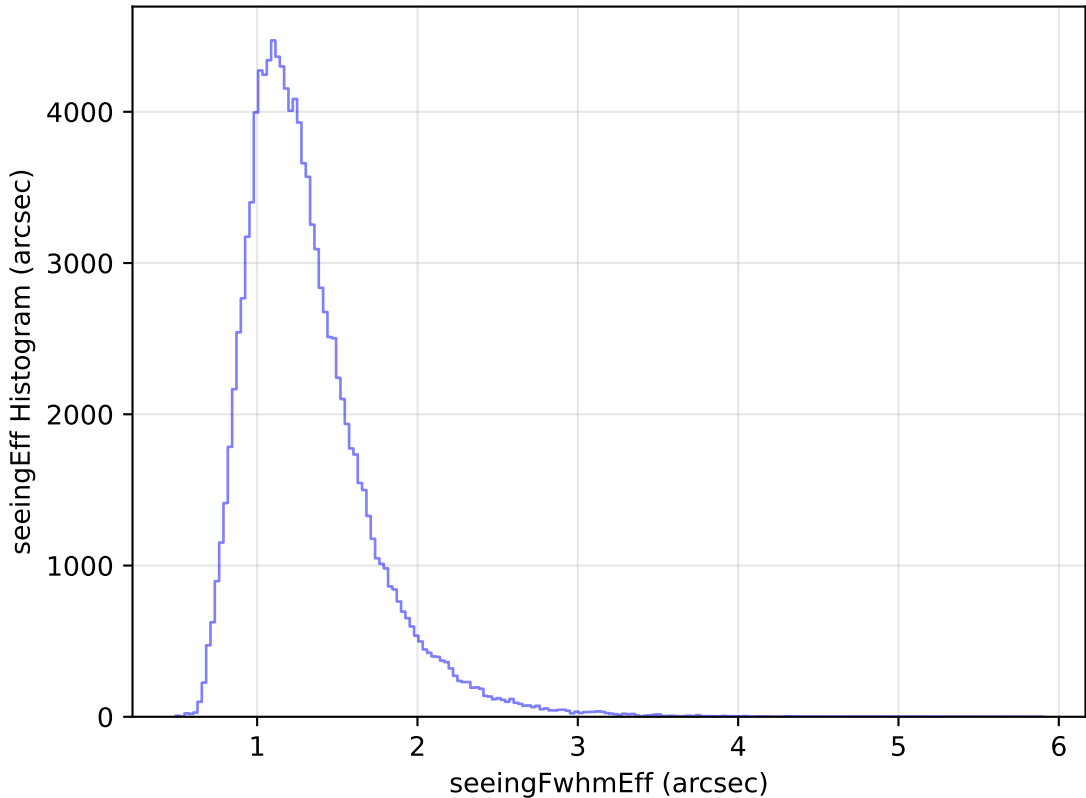
too_elab_heavy_r64_d3_gz_v3.4_10yrs All sky u band: seeingEff Histogram
