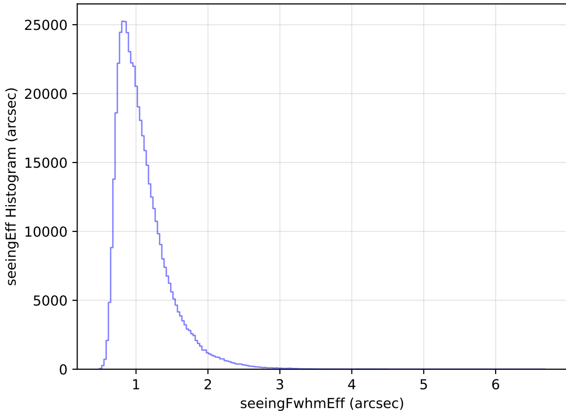
too_elab_heavy_r64_d3_gz_v3.4_10yrs All sky i band: seeingEff Histogram
