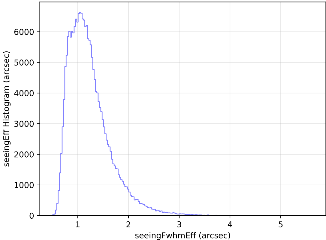
too_elab_heavy_r64_d3_gz_v3.4_10yrs All sky g band: seeingEff Histogram
