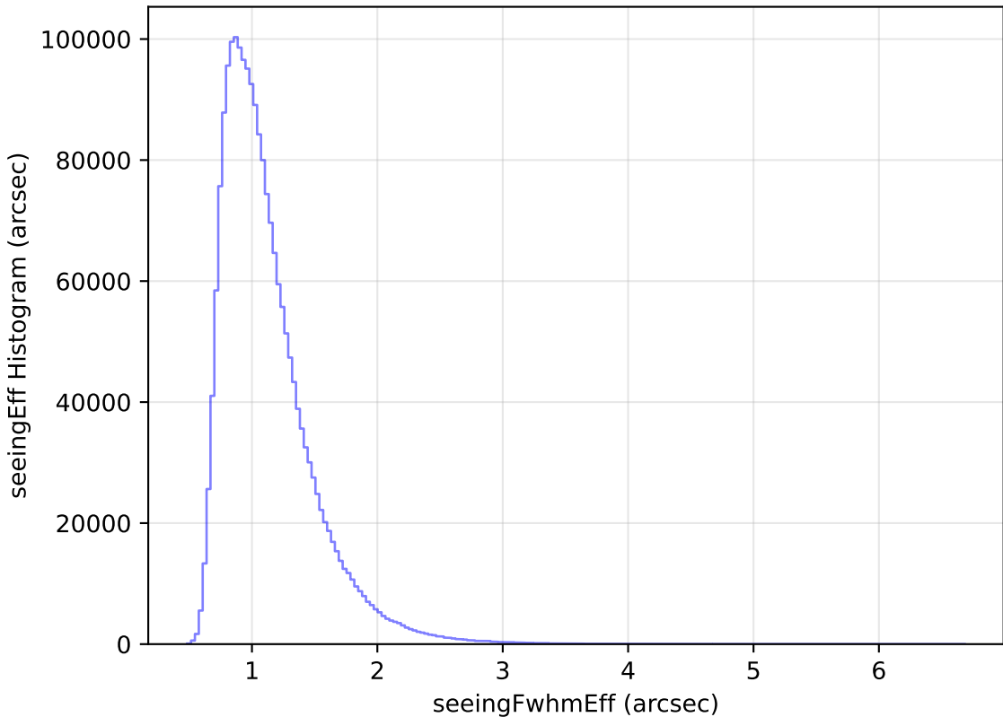
too_elab_heavy_r64_d3_gz_v3.4_10yrs All sky all bands: seeingEff Histogram
