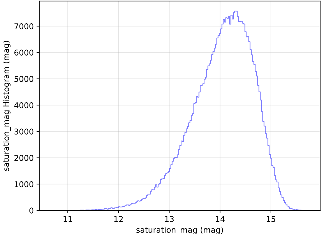
too_elab_heavy_r64_d3_gz_v3.4_10yrs WFD z band: saturation_mag Histogram
