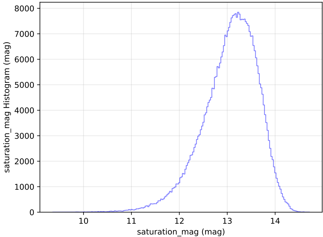
too_elab_heavy_r64_d3_gz_v3.4_10yrs WFD y band: saturation_mag Histogram
