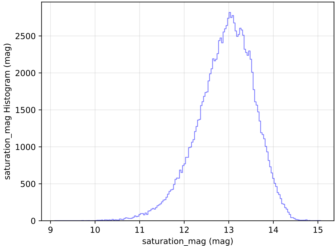
too_elab_heavy_r64_d3_gz_v3.4_10yrs WFD u band: saturation_mag Histogram
