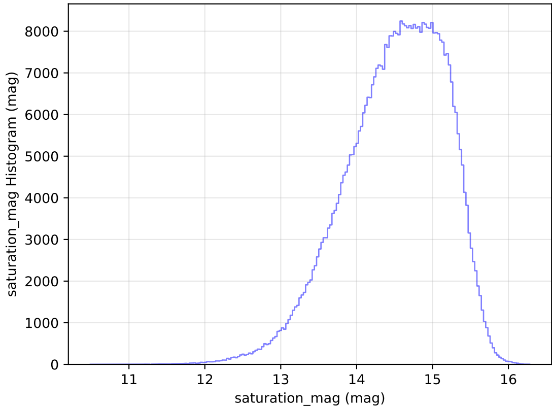
too_elab_heavy_r64_d3_gz_v3.4_10yrs WFD r band: saturation_mag Histogram
