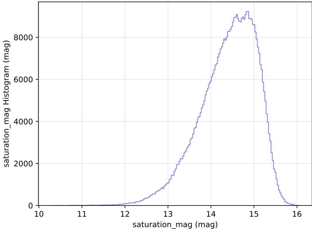
too_elab_heavy_r64_d3_gz_v3.4_10yrs WFD i band: saturation_mag Histogram
