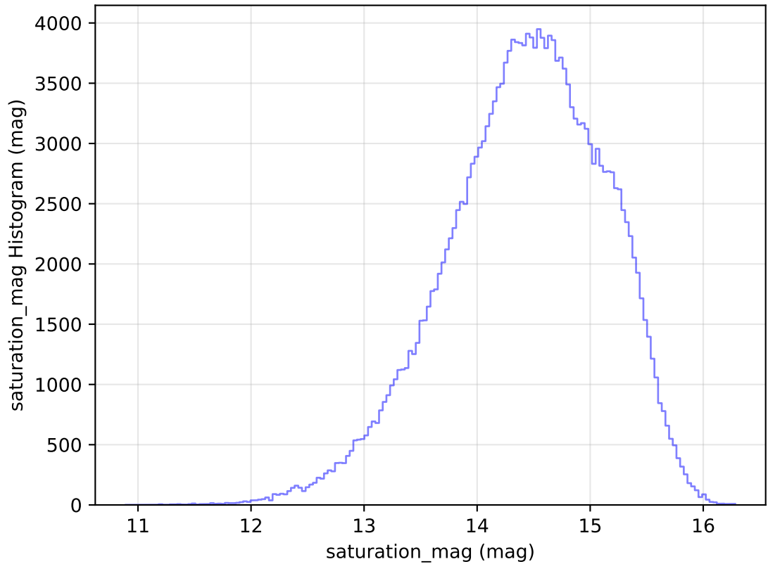
too_elab_heavy_r64_d3_gz_v3.4_10yrs WFD g band: saturation_mag Histogram
