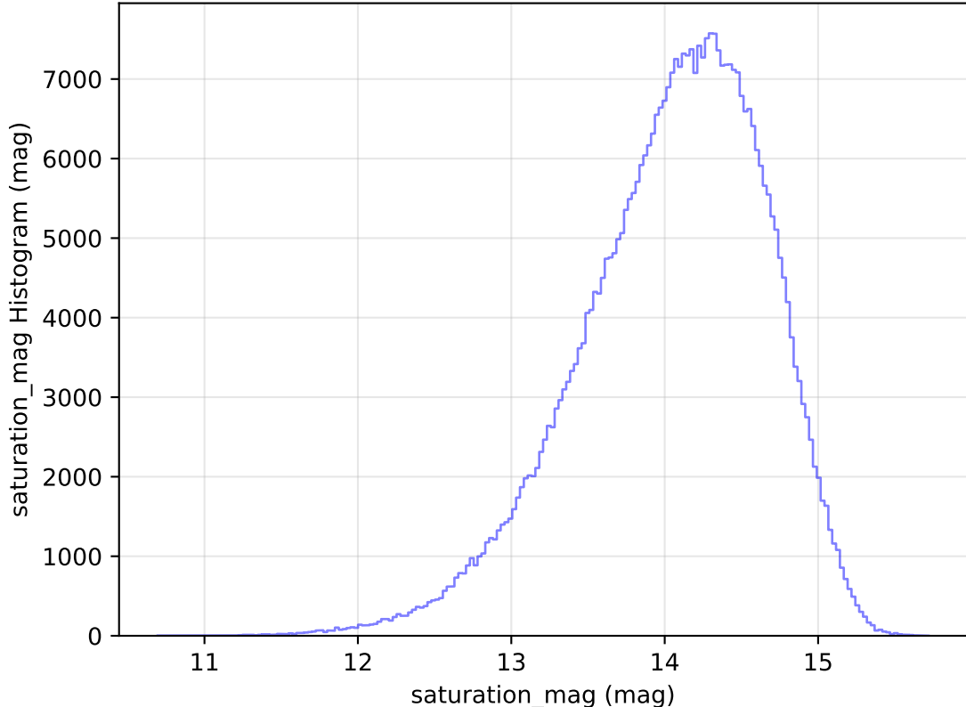
too_elab_heavy_r64_d3_gz_v3.4_10yrs All sky z band: saturation_mag Histogram
