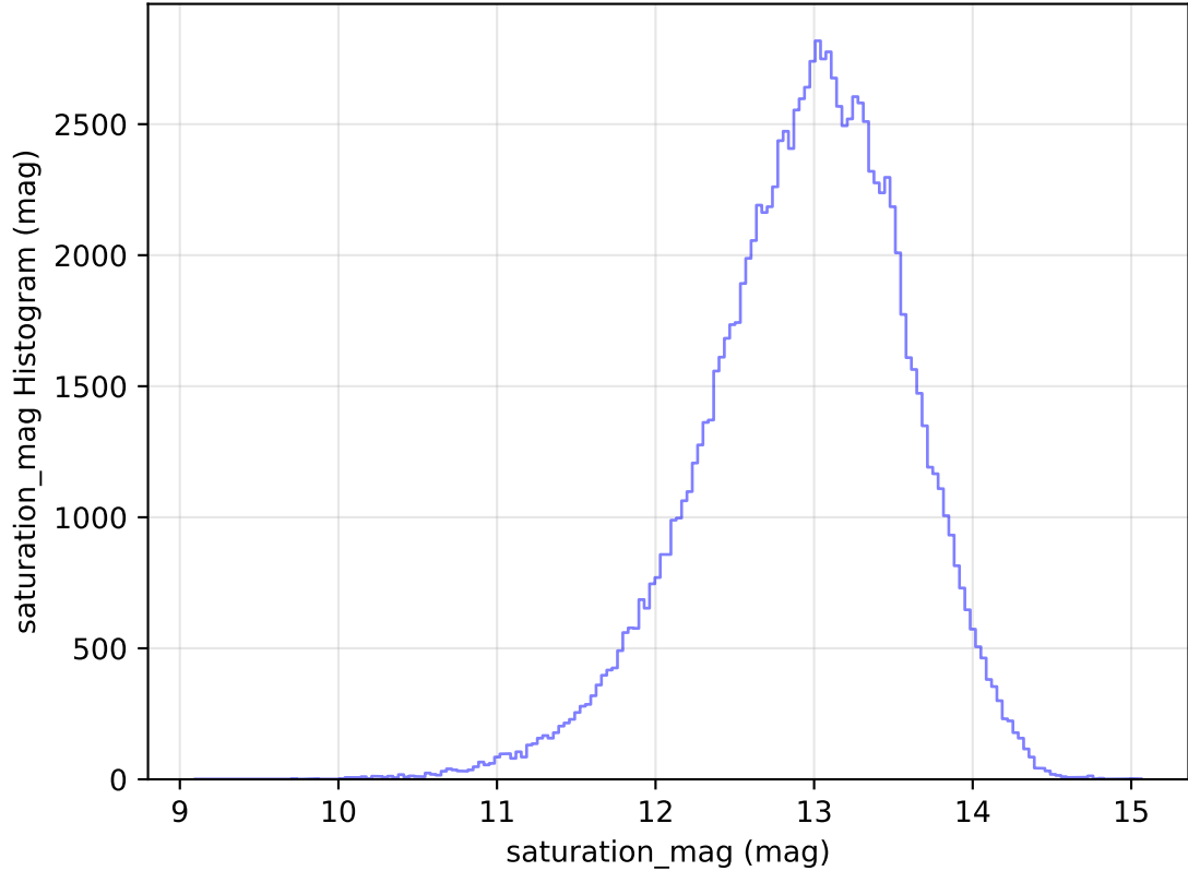
too_elab_heavy_r64_d3_gz_v3.4_10yrs All sky u band: saturation_mag Histogram
