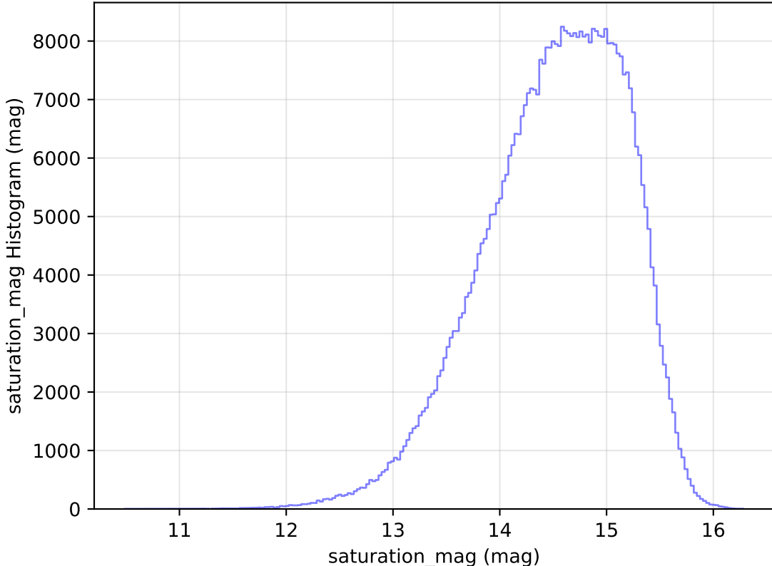
too_elab_heavy_r64_d3_gz_v3.4_10yrs All sky r band: saturation_mag Histogram
