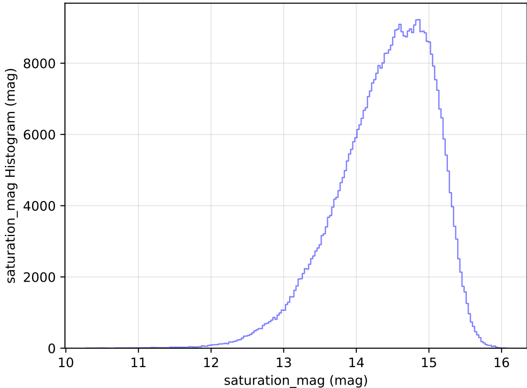
too_elab_heavy_r64_d3_gz_v3.4_10yrs All sky i band: saturation_mag Histogram
