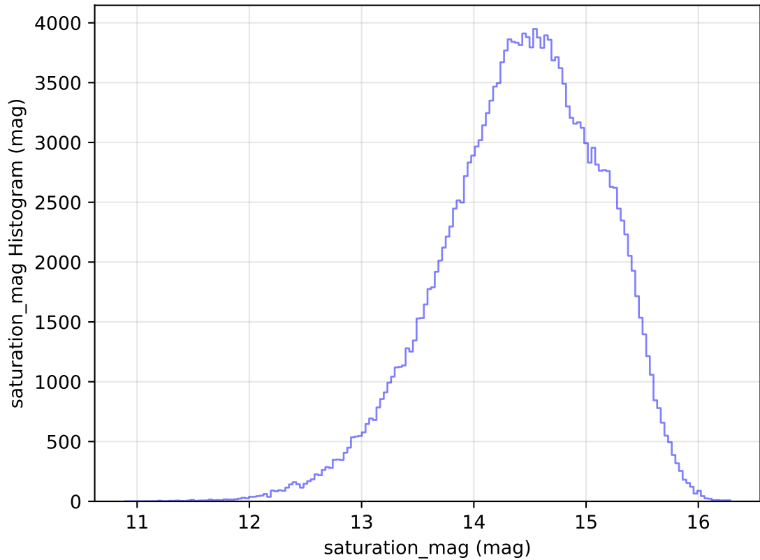
too_elab_heavy_r64_d3_gz_v3.4_10yrs All sky g band: saturation_mag Histogram
