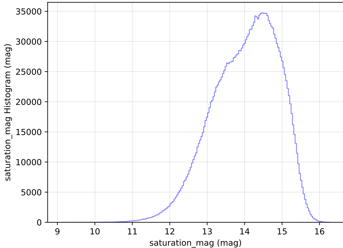
too_elab_heavy_r64_d3_gz_v3.4_10yrs All sky all bands: saturation_mag Histogram
