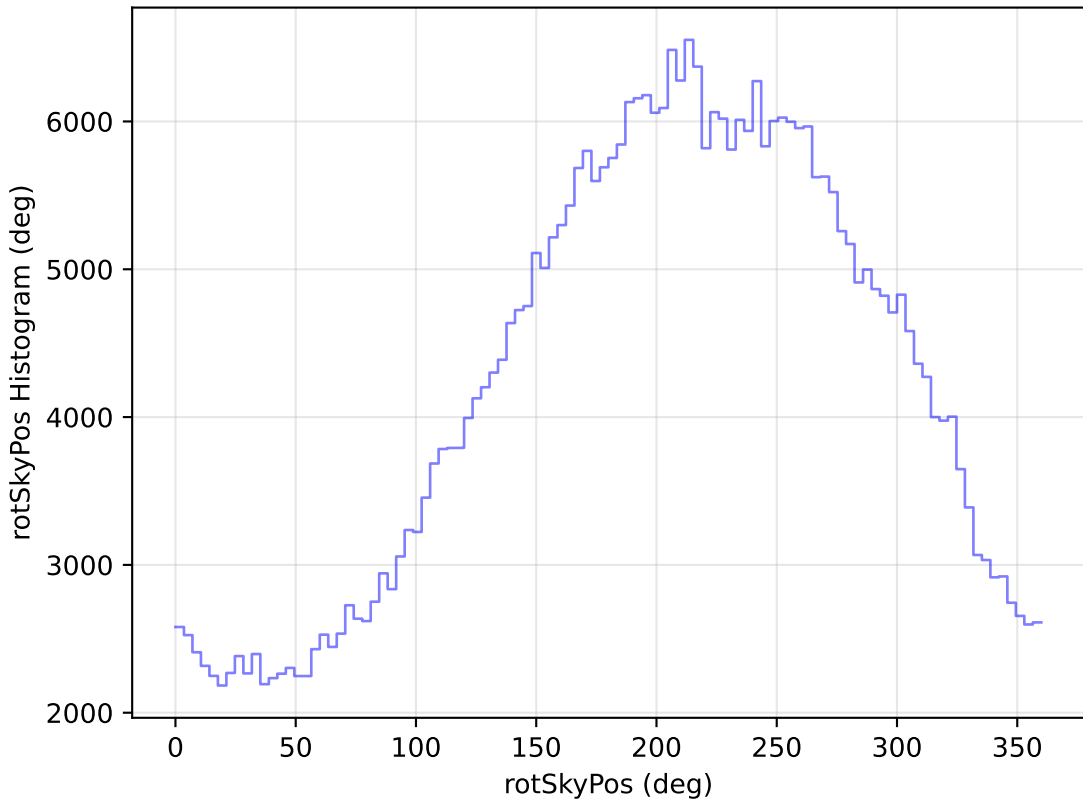
too_elab_heavy_r64_d3_gz_v3.4_10yrs WFD z band: rotSkyPos Histogram
