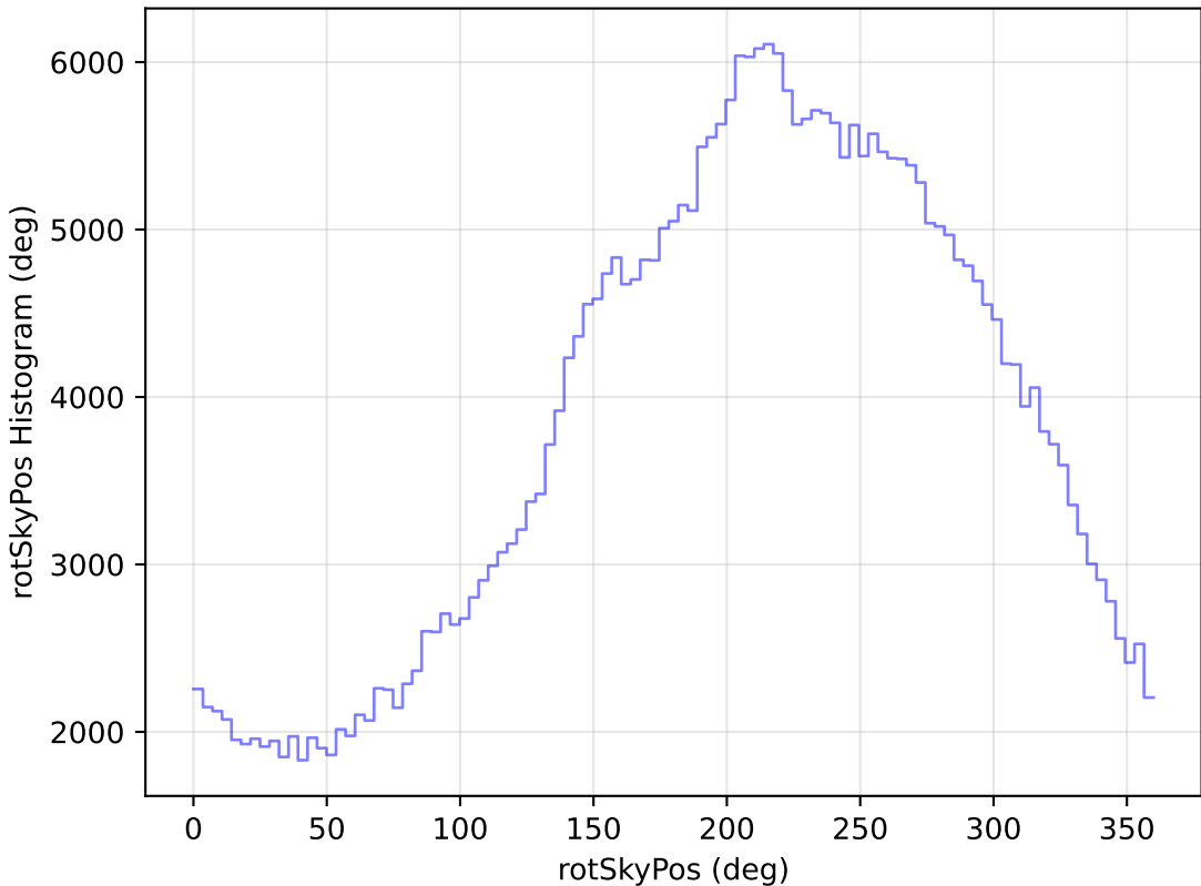
too_elab_heavy_r64_d3_gz_v3.4_10yrs WFD y band: rotSkyPos Histogram
