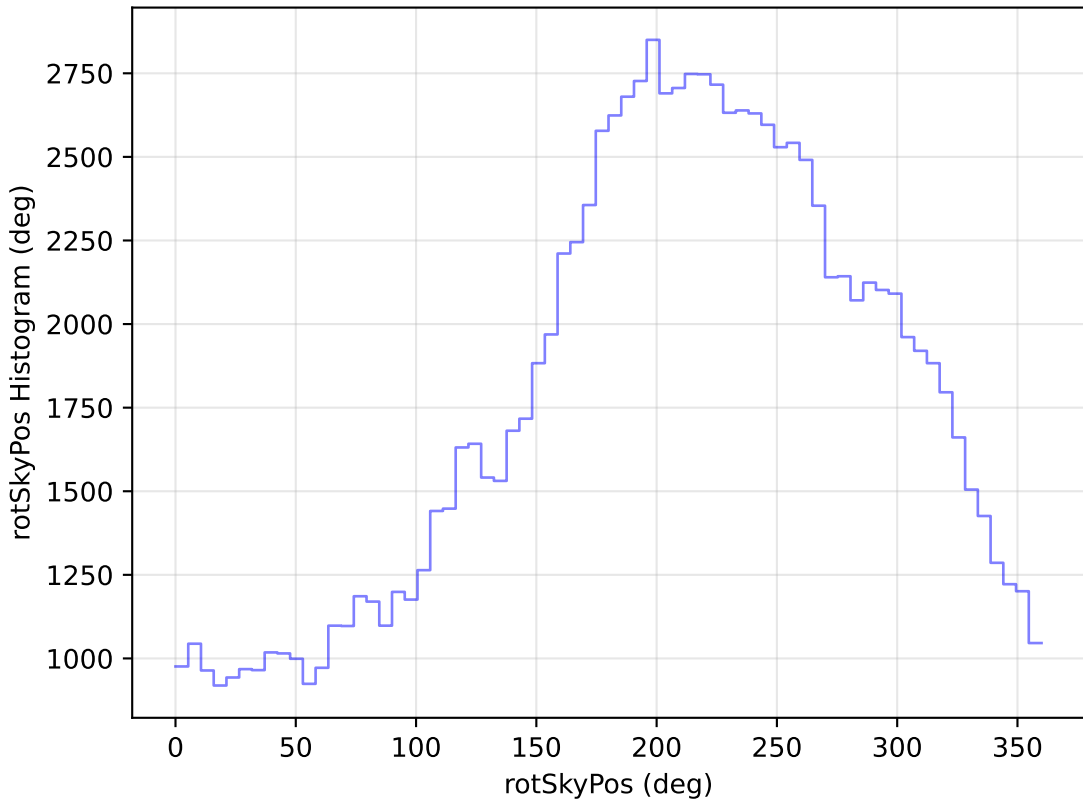
too_elab_heavy_r64_d3_gz_v3.4_10yrs WFD u band: rotSkyPos Histogram
