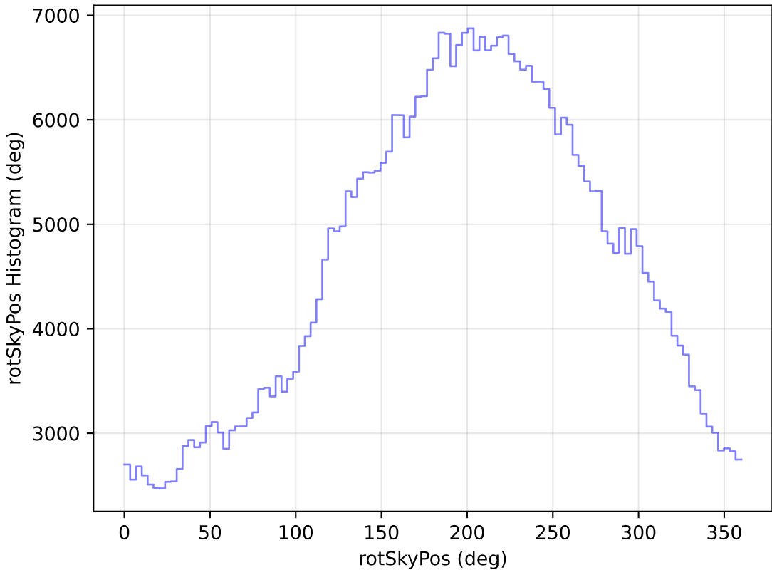
too_elab_heavy_r64_d3_gz_v3.4_10yrs WFD r band: rotSkyPos Histogram
