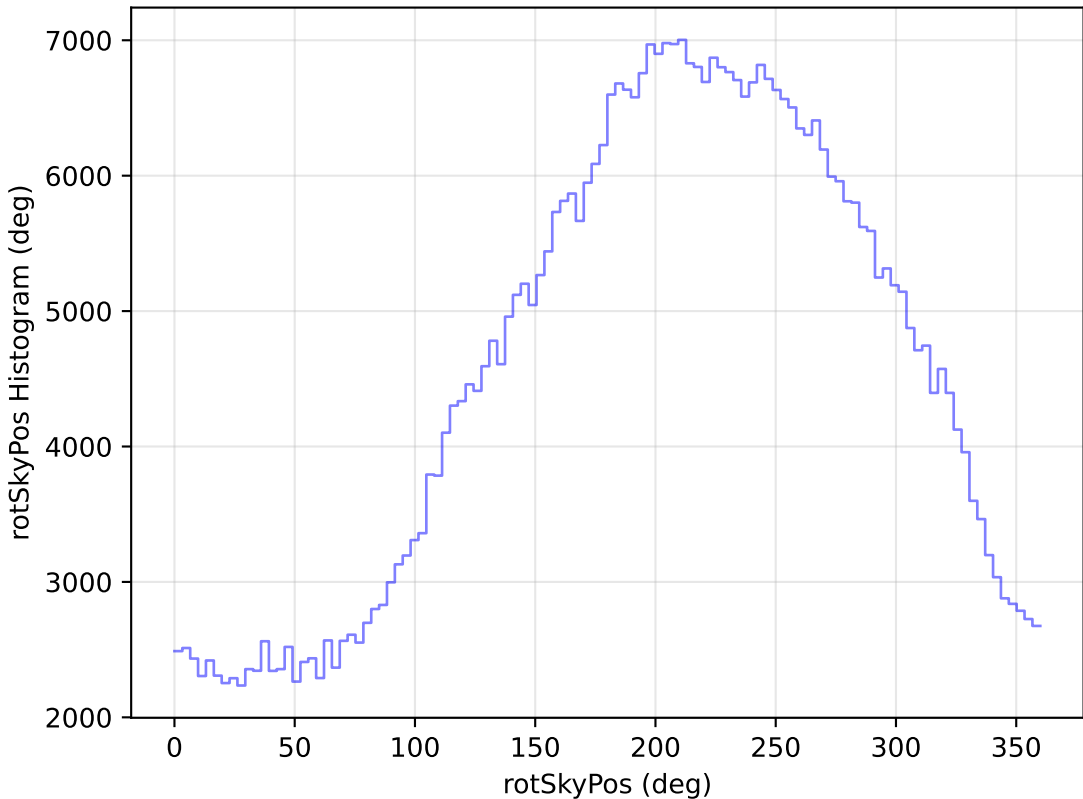
too_elab_heavy_r64_d3_gz_v3.4_10yrs WFD i band: rotSkyPos Histogram
