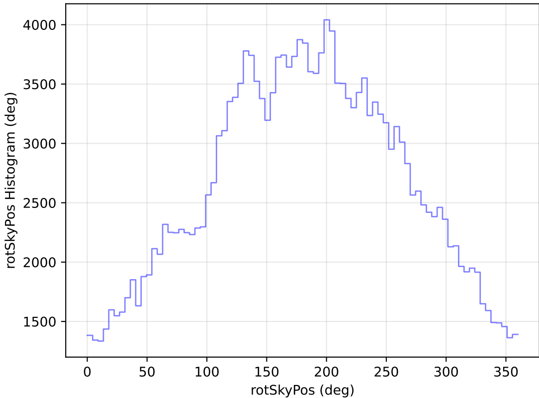
too_elab_heavy_r64_d3_gz_v3.4_10yrs WFD g band: rotSkyPos Histogram
