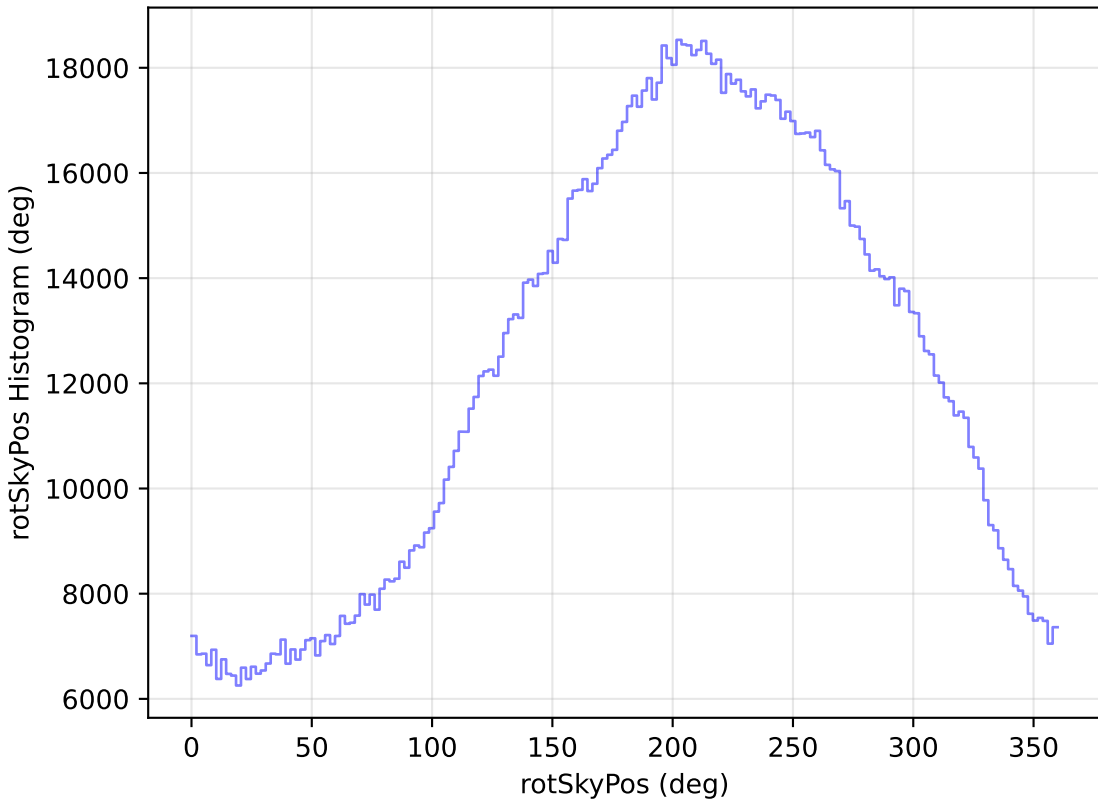
too_elab_heavy_r64_d3_gz_v3.4_10yrs WFD all bands: rotSkyPos Histogram
