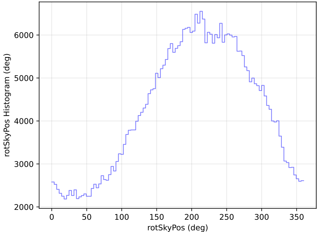
too_elab_heavy_r64_d3_gz_v3.4_10yrs All sky z band: rotSkyPos Histogram
