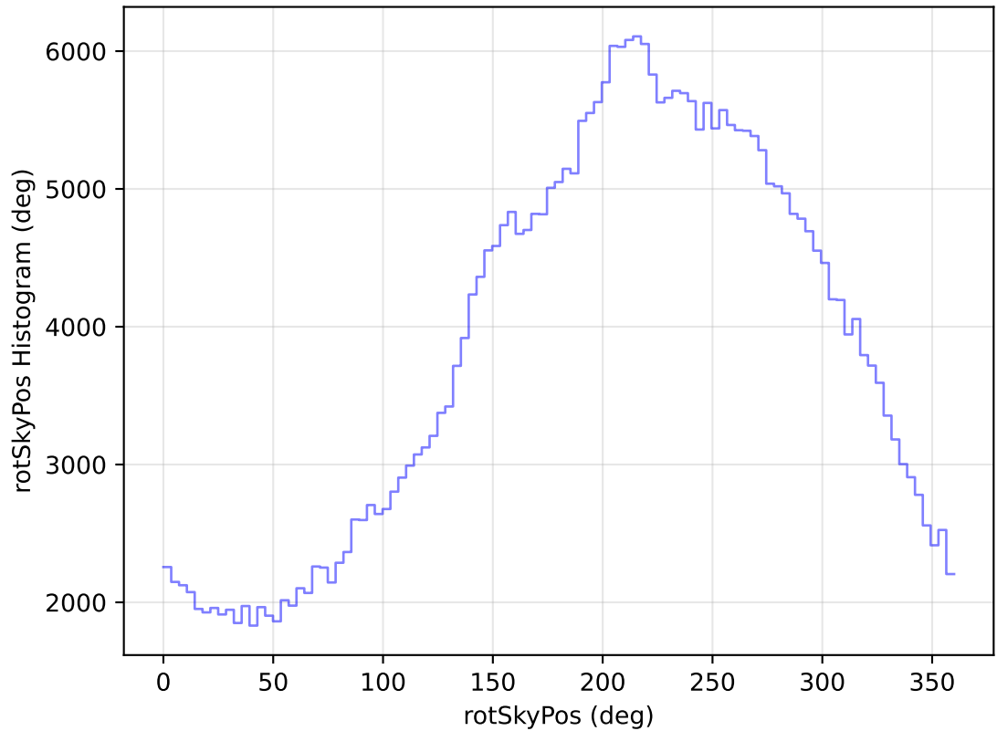
too_elab_heavy_r64_d3_gz_v3.4_10yrs All sky y band: rotSkyPos Histogram
