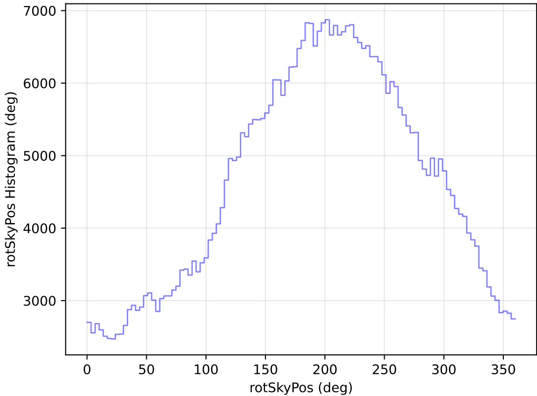
too_elab_heavy_r64_d3_gz_v3.4_10yrs All sky r band: rotSkyPos Histogram
