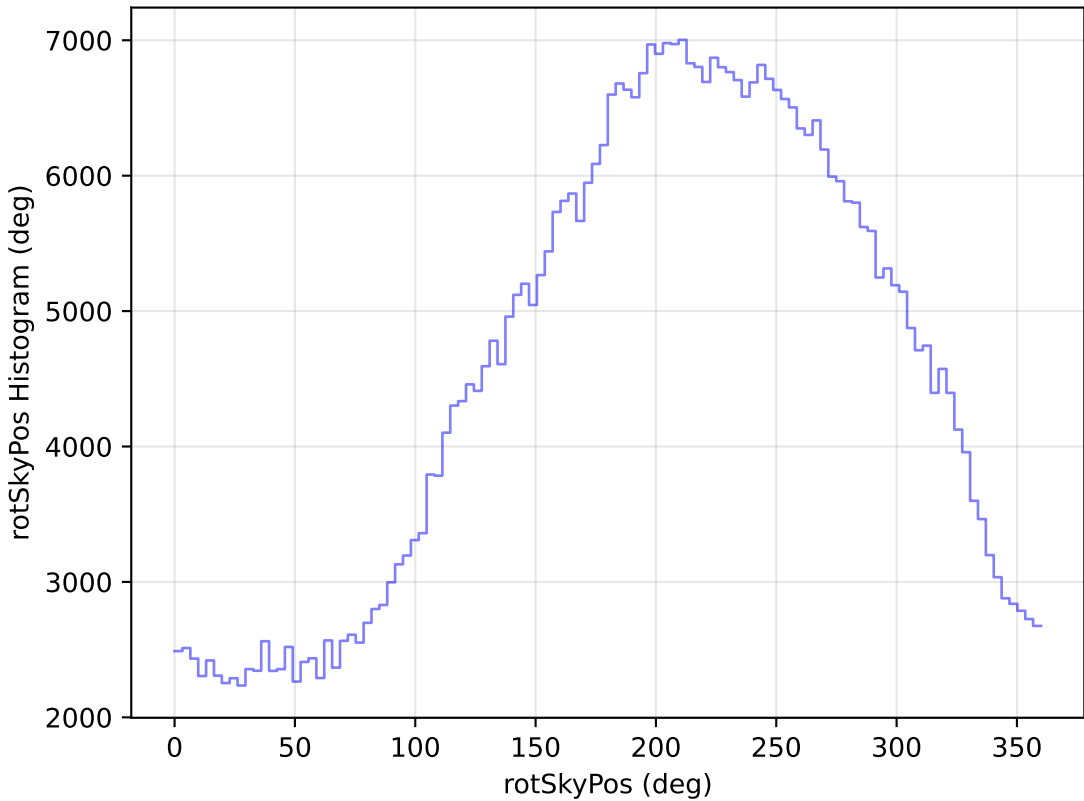
too_elab_heavy_r64_d3_gz_v3.4_10yrs All sky i band: rotSkyPos Histogram
