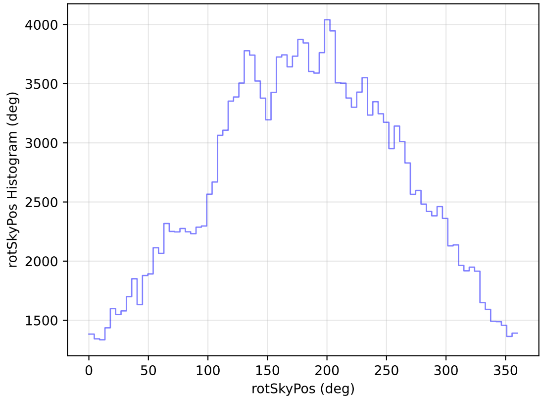
too_elab_heavy_r64_d3_gz_v3.4_10yrs All sky g band: rotSkyPos Histogram
