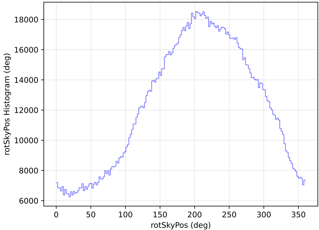
too_elab_heavy_r64_d3_gz_v3.4_10yrs All sky all bands: rotSkyPos Histogram
