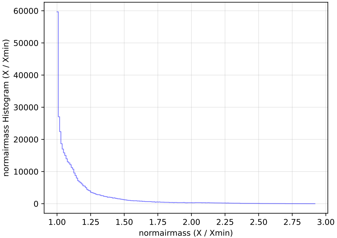
too_elab_heavy_r64_d3_gz_v3.4_10yrs WFD z band: normairmass Histogram
