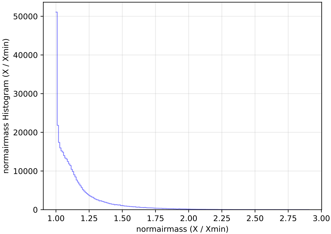
too_elab_heavy_r64_d3_gz_v3.4_10yrs WFD y band: normairmass Histogram
