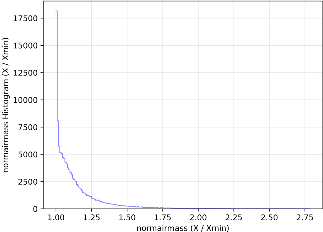
too_elab_heavy_r64_d3_gz_v3.4_10yrs WFD u band: normairmass Histogram
