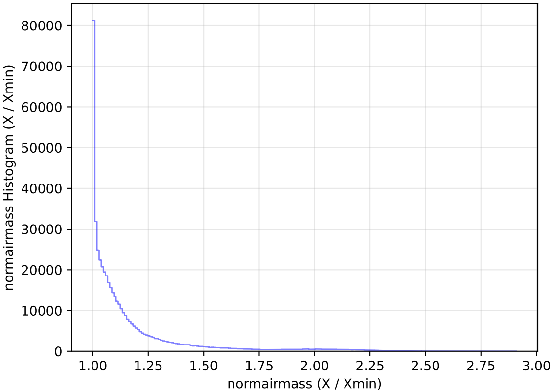
too_elab_heavy_r64_d3_gz_v3.4_10yrs WFD r band: normairmass Histogram
