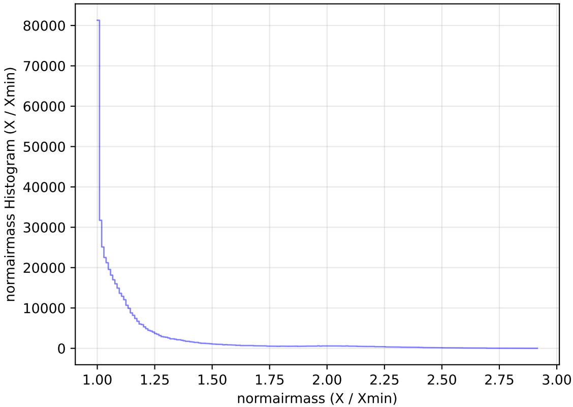
too_elab_heavy_r64_d3_gz_v3.4_10yrs WFD i band: normairmass Histogram
