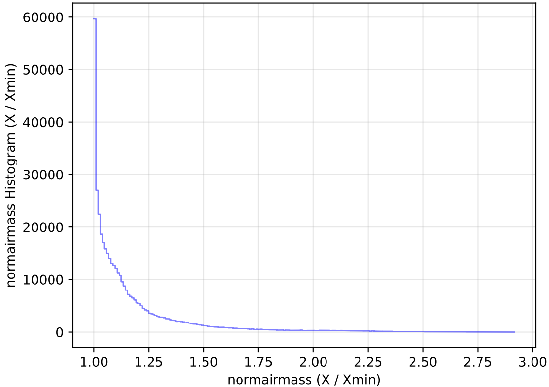
too_elab_heavy_r64_d3_gz_v3.4_10yrs All sky z band: normairmass Histogram
