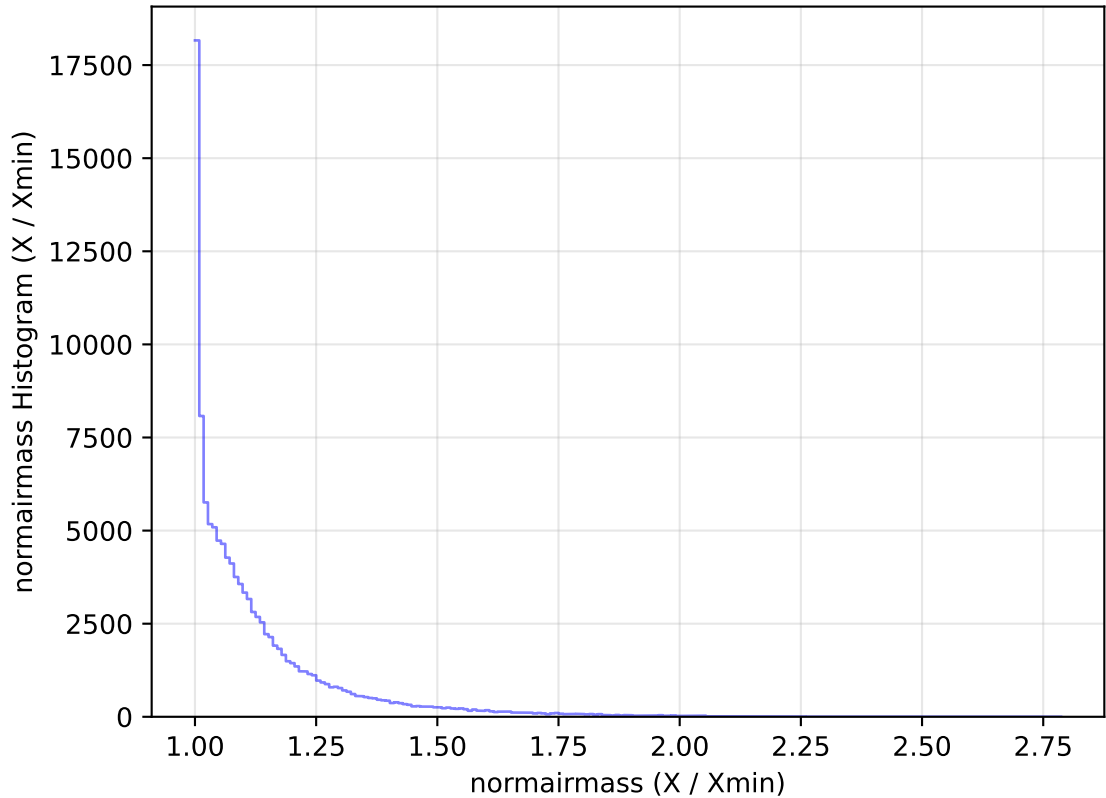
too_elab_heavy_r64_d3_gz_v3.4_10yrs All sky u band: normairmass Histogram
