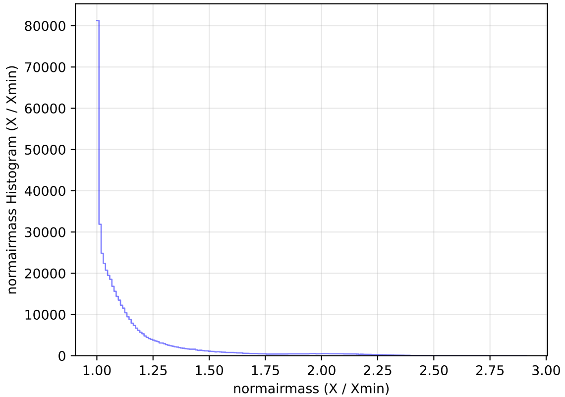
too_elab_heavy_r64_d3_gz_v3.4_10yrs All sky r band: normairmass Histogram
