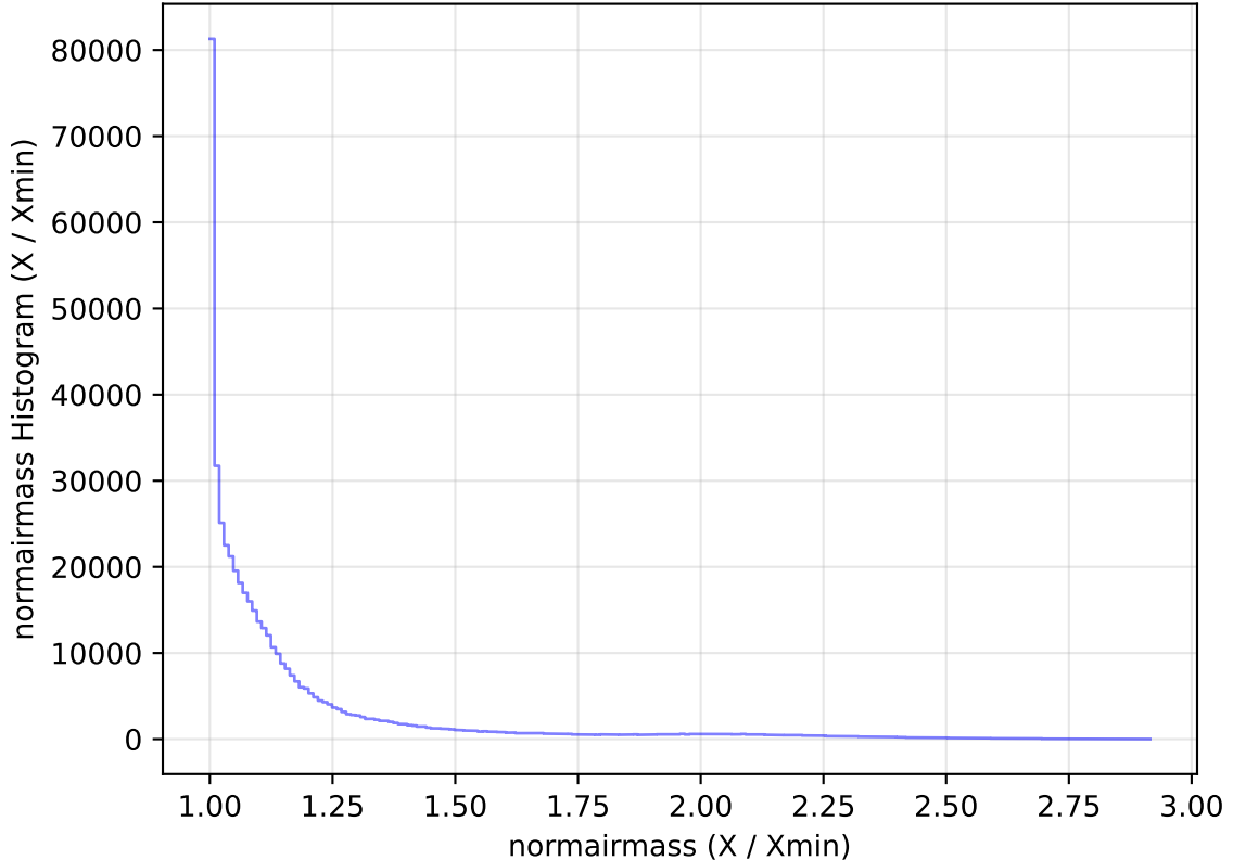
too_elab_heavy_r64_d3_gz_v3.4_10yrs All sky i band: normairmass Histogram
