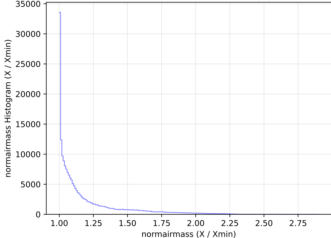
too_elab_heavy_r64_d3_gz_v3.4_10yrs All sky g band: normairmass Histogram
