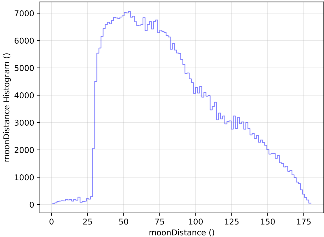
too_elab_heavy_r64_d3_gz_v3.4_10yrs WFD z band: moonDistance Histogram
